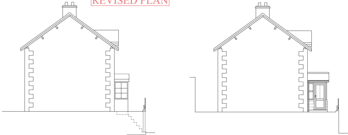
West Elevation Existing.
